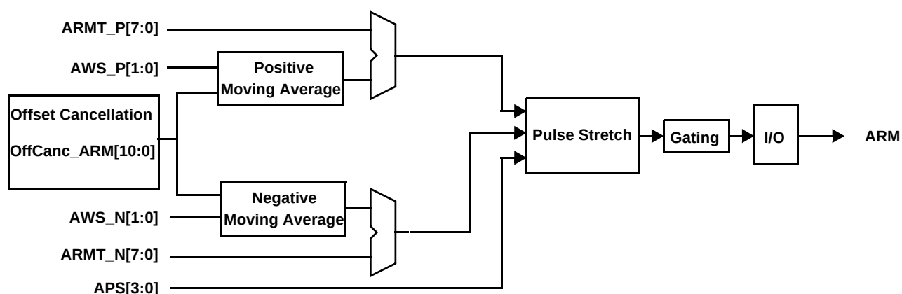
Figure 24. Arming Function Block Diagram - Moving Average Mode
