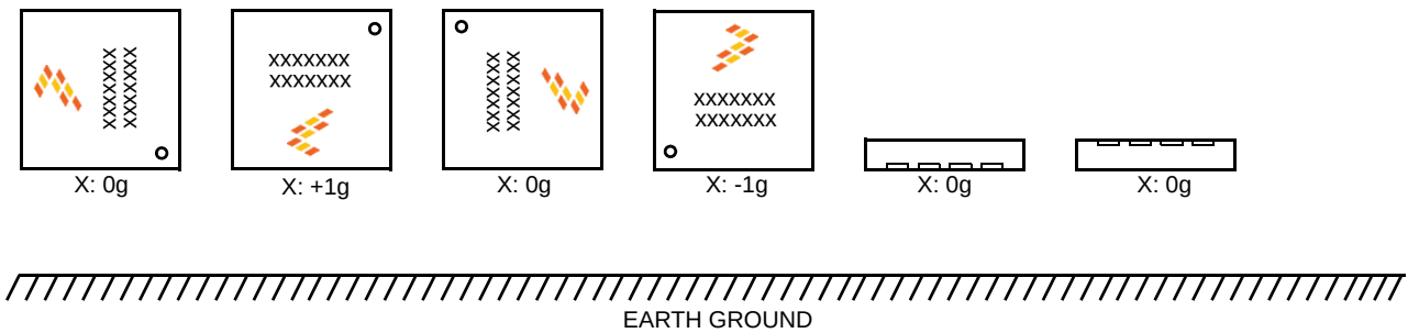
Figure 2. Device Orientation Diagram
