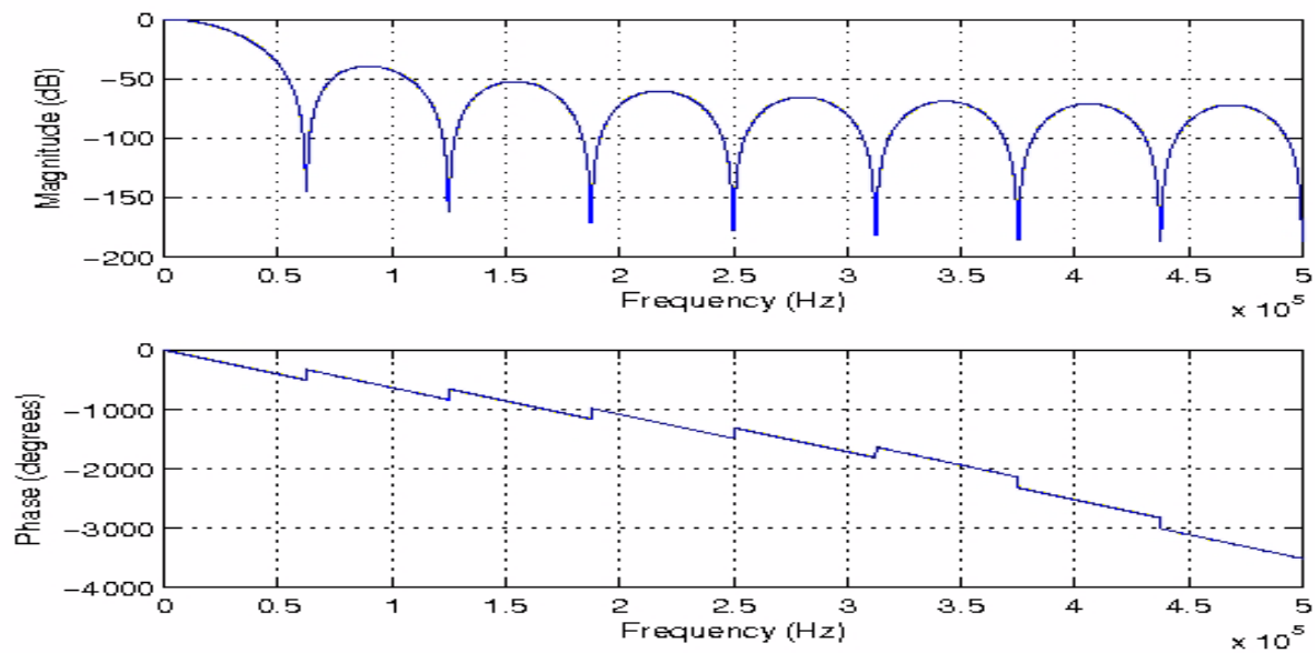
Figure 13. Sinc Filter Response, t_s = 8 \mu s
